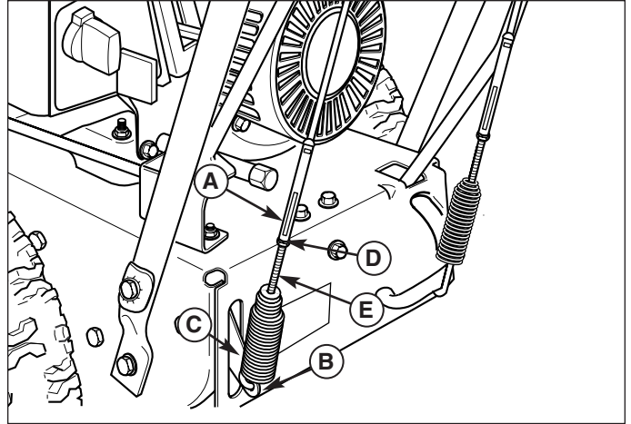
Figure 20. Traction Drive Adjustment
